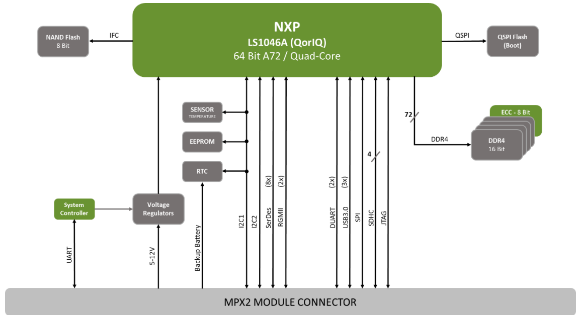
Figure 3-1 Block Diagram
