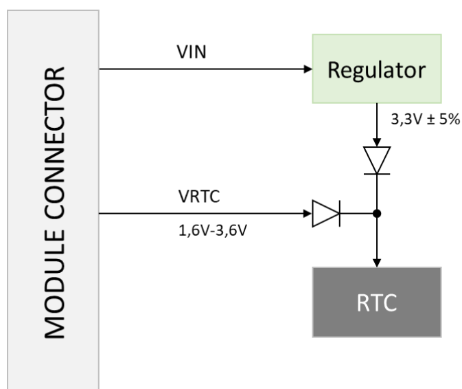
Figure 4-4 RTC: buffering
