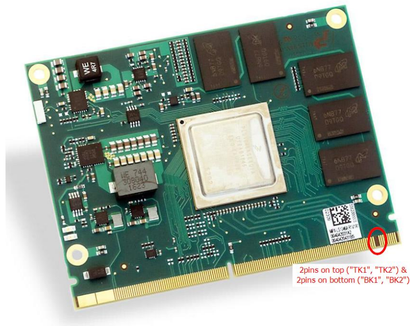
Figure 5-1 Additional Key Pins
