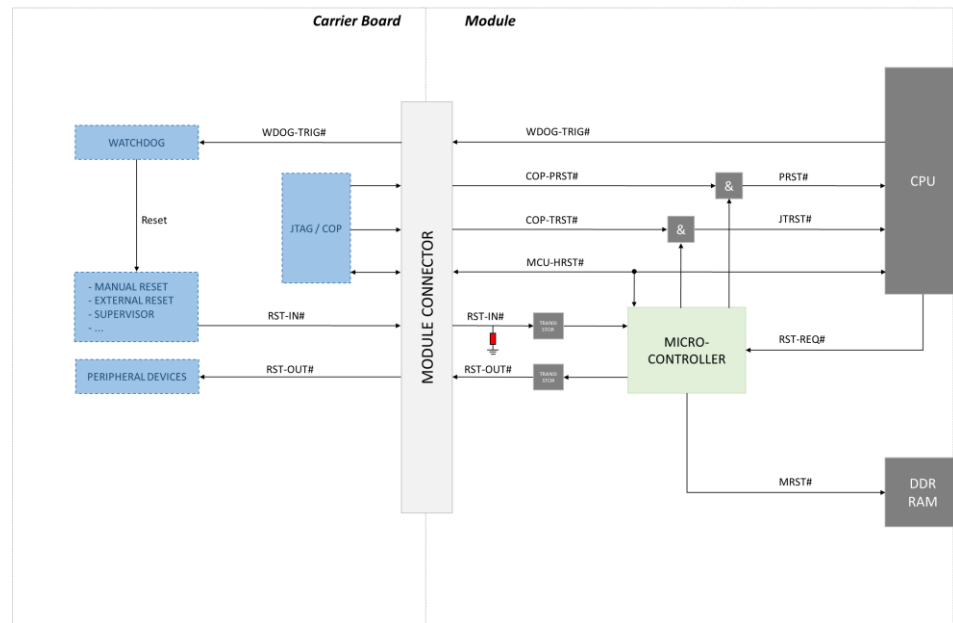
Figure 4-1 Reset Structure
