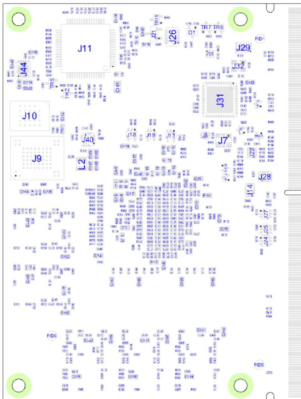
Figure 5-8 Bottom Components
