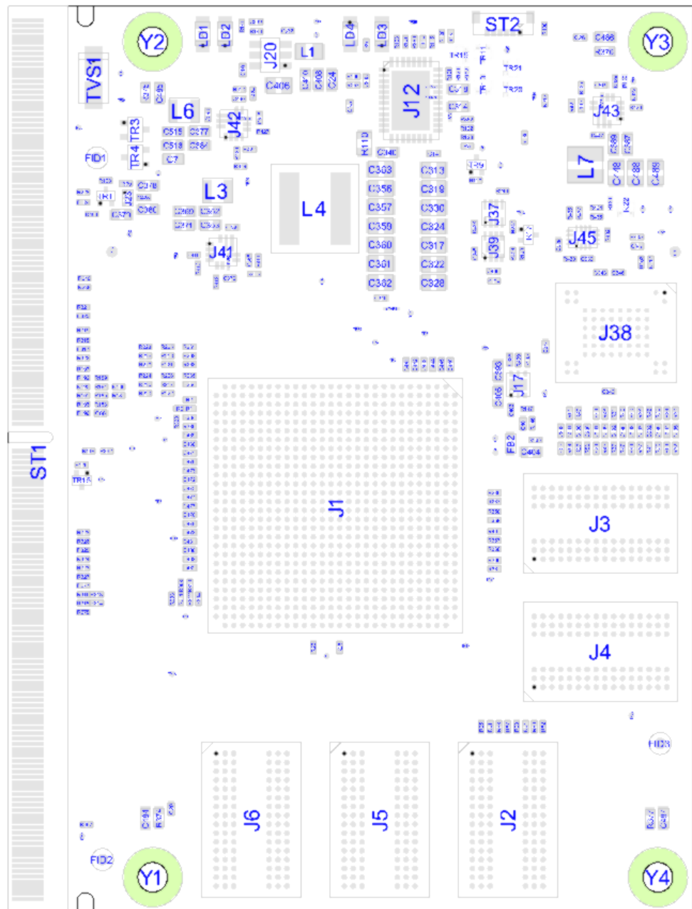
Figure 5-7 Top Components
