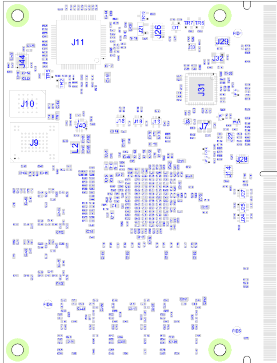
Figure 5-8 Bottom Components
