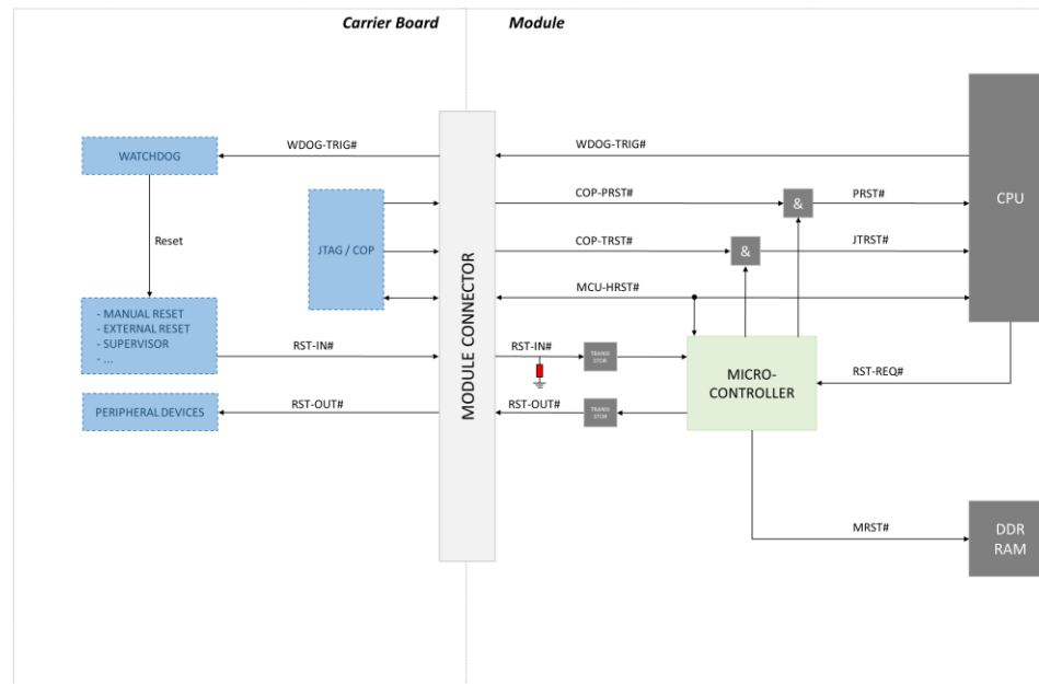
Figure 4-1 Reset Structure
