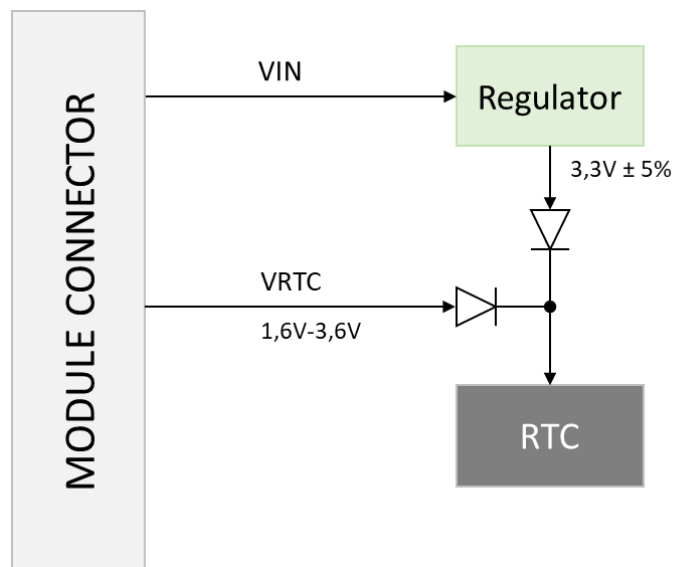
Figure 4-4 RTC: buffering
