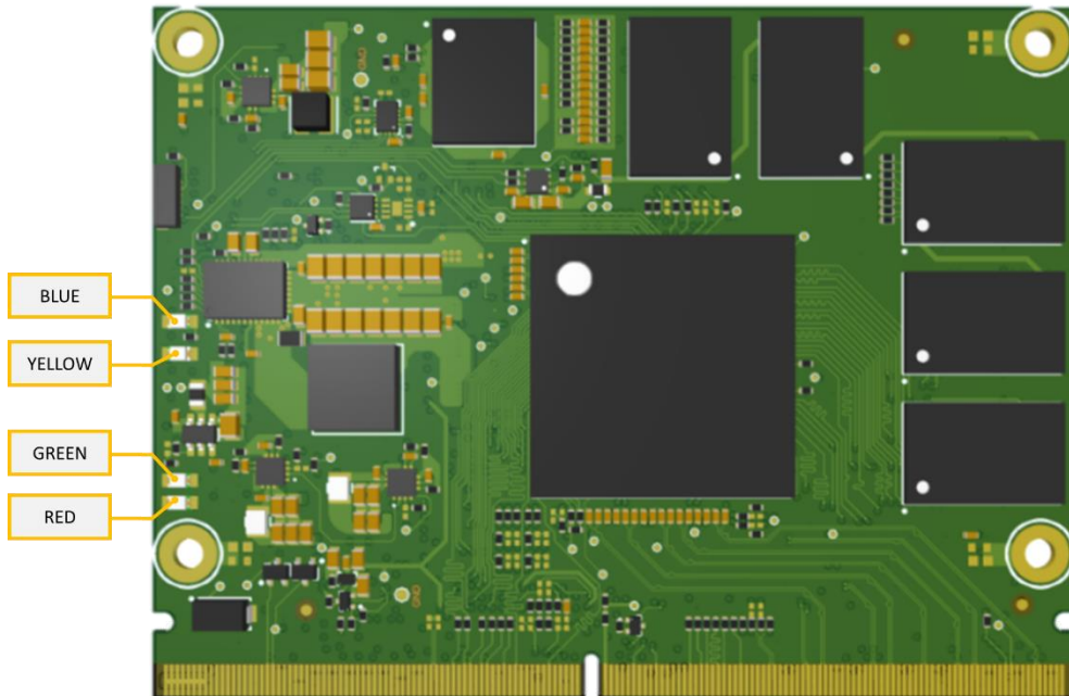
Figure 4-3 LEDs
