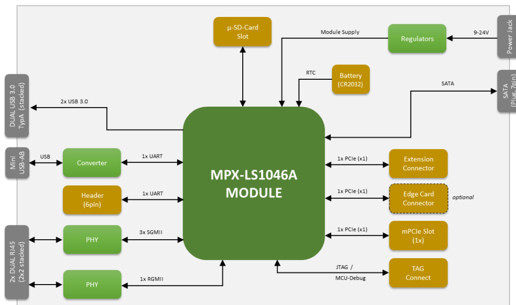
Graphic 1: SBC-LS1046A Block Diagram
