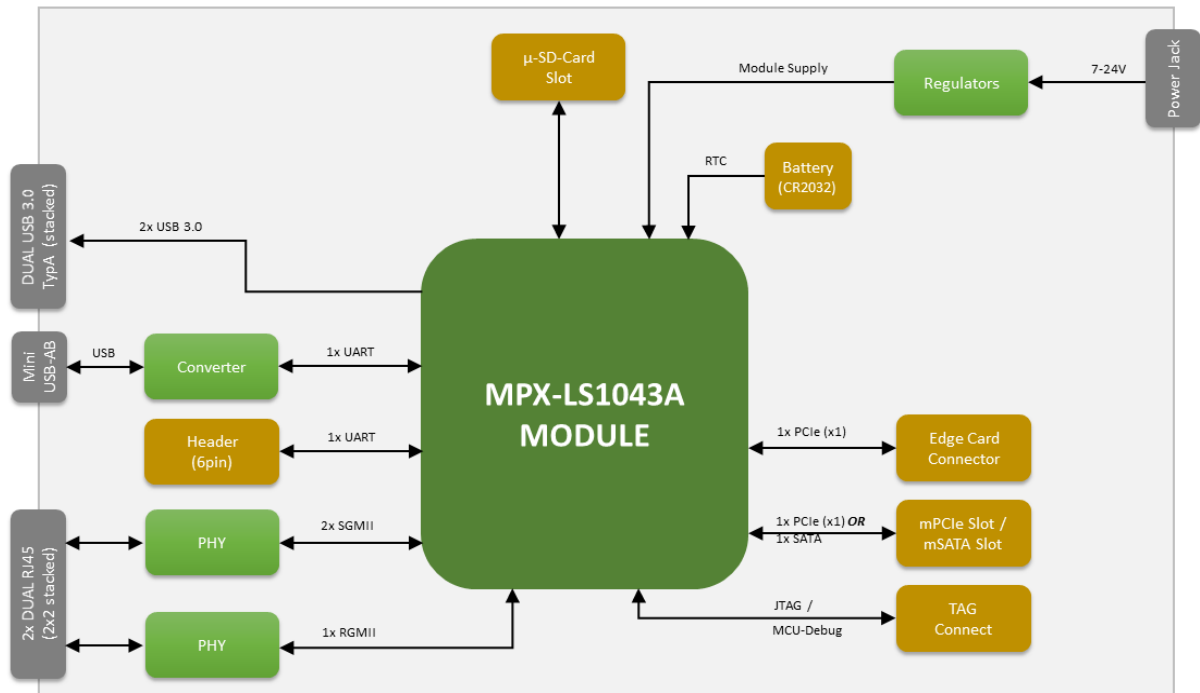
Graphic 1: SBC-LS1043A Block Diagram
